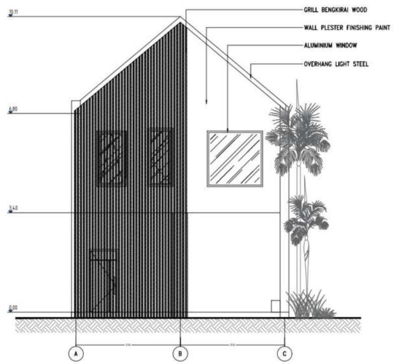
FRONT ELEVATION
