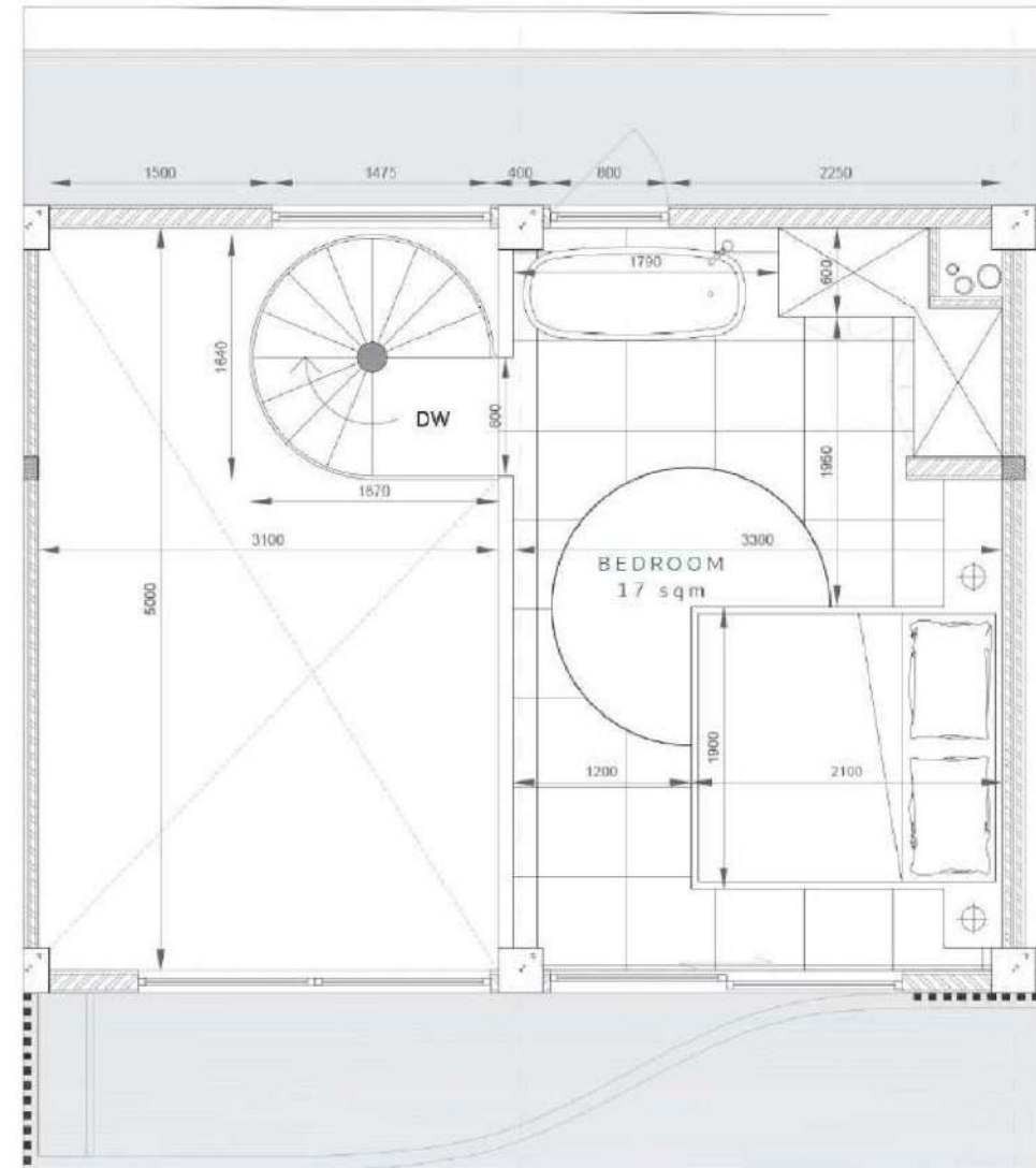
MEZZANINE PLAN
