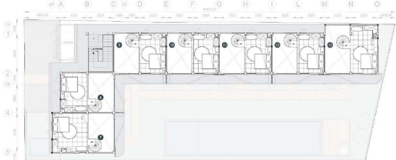
FLOOR PLAN | SF MEZZANINE
